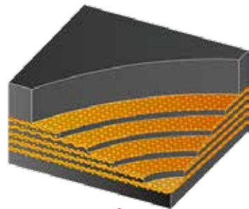
MULTI-PLY BELTING
